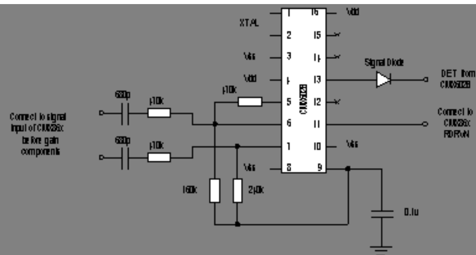
CMX602B circuit configuration
