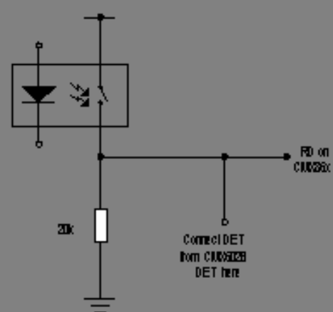
Optoisolated Ring Detect on CMX86x
