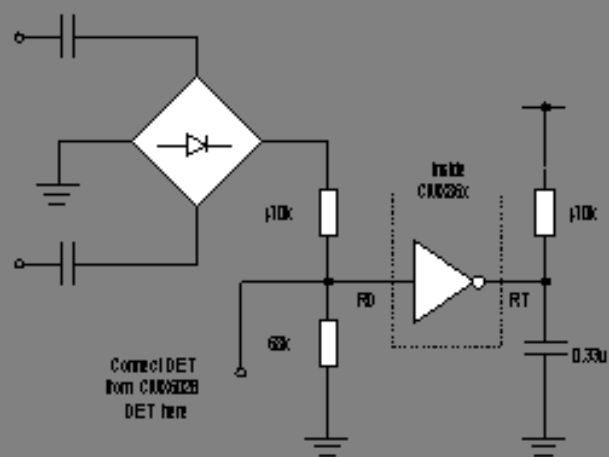
AC coupled bridge Ring Detect on CMX86x
